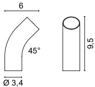
7504 45° expanding bend
