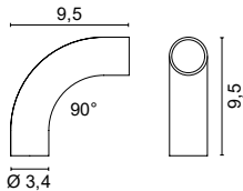
7500 90° expanding bend
