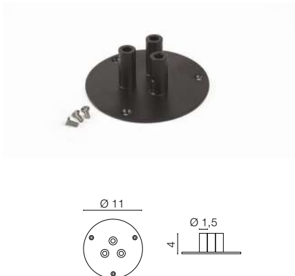
0252/3 Installation base for 3 art. Trilli
