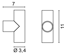
7501 T Joint expanding bend
