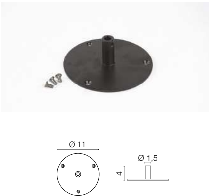
0252/1 Installation base for 1 art. Trilli
